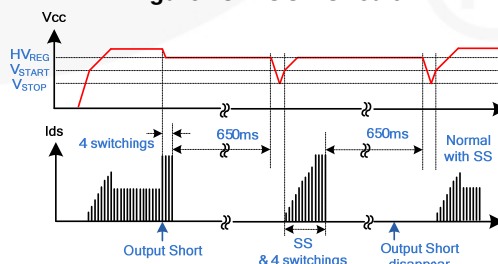
Figure 24. AOCP Waveform
