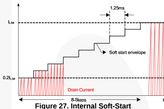
Figure 27. Internal Soft-Start
