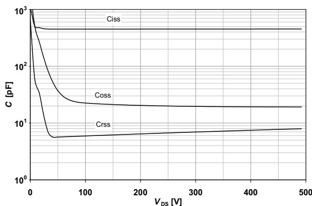
Figure 66 Typ. capacitances; C = f(V_{DS}) , V_{GS} = 0V , f = 1MHz
