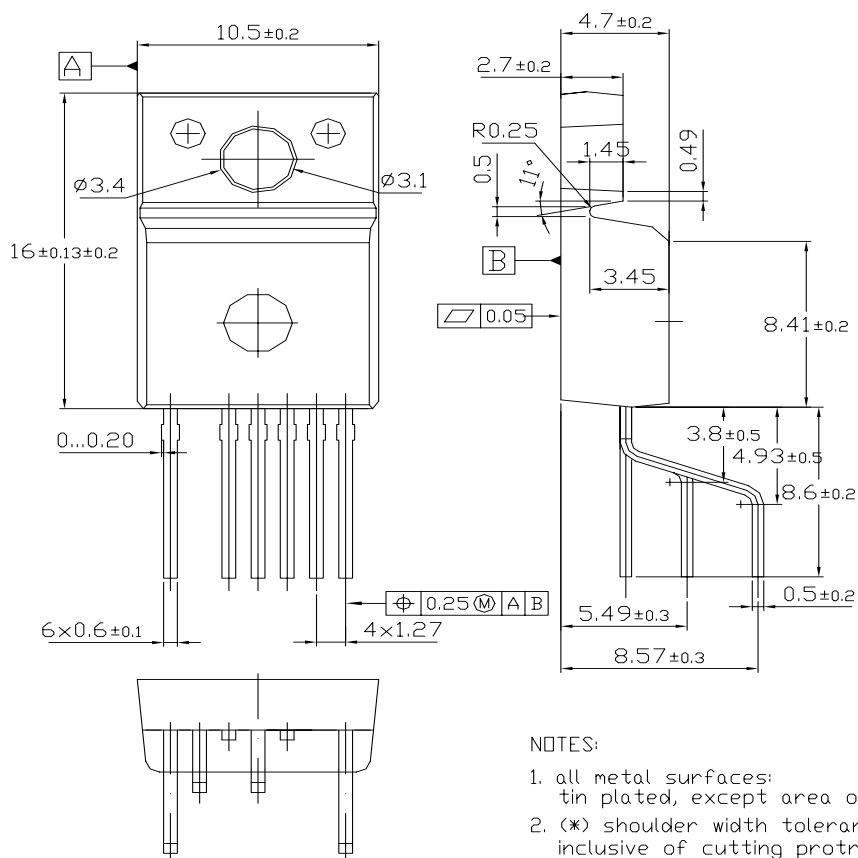
Figure 70 PG-TO220-6-247 (PB-free Plating FullPak Package)
