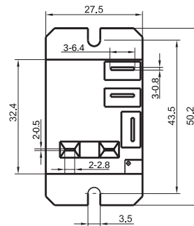
Outline Dimensions
