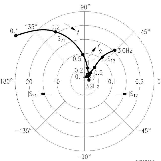
S 12 , S 21 = f ( f ) I C = 20 mA, V CE = 10 V, Z 0 = 50 Ω
