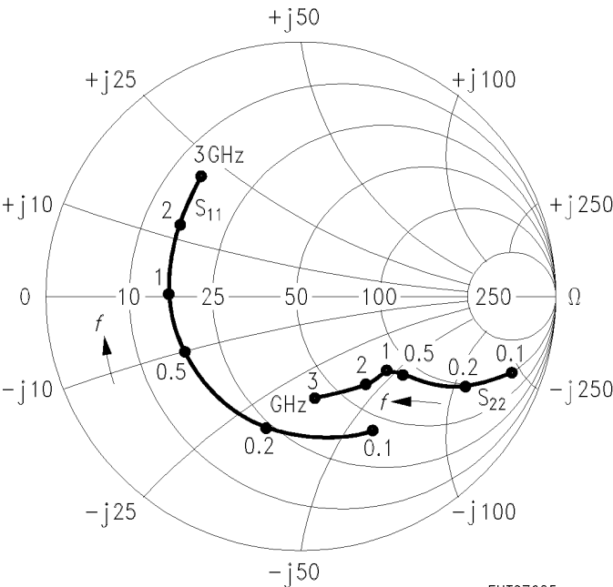
S 11 , S 22 = f ( f ) I C = 20 mA, V CE = 10 V, Z 0 = 50 Ω
