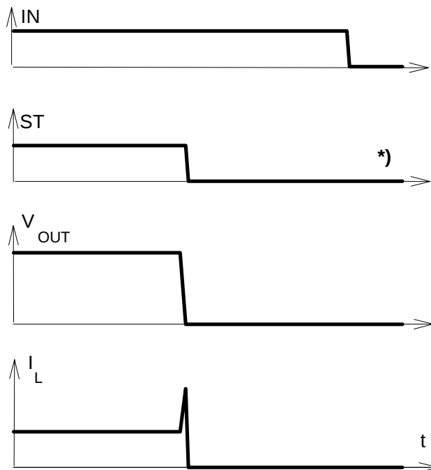
Figure 4a: Overtemperature:
