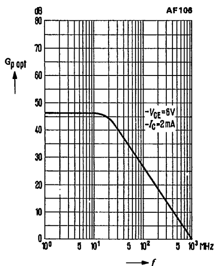
Optimum power gain G_{p, opt} = f(f) -V_{CE} = 6V ; -I_C = 2mA (common emitter configuration)
