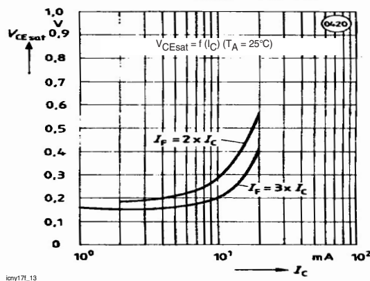
Figure 13. Saturation Voltage vs. Collector Current and Modulation Depth CNY17F-2
