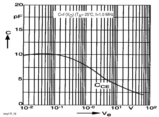
Figure 19. Transistor Capacitance
