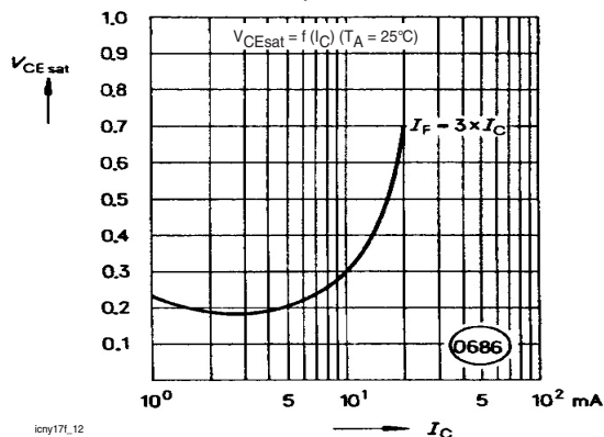
Figure 12. Saturation Voltage vs. Collector Current and Modulation Depth CNY17F-1
