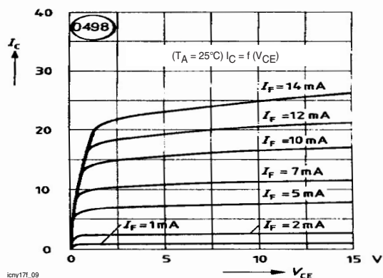
Figure 9. Output Characteristics CNY17F-2, -3
