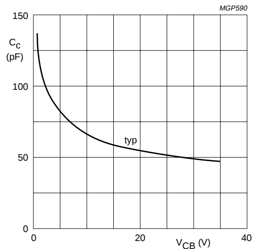
Fig.6 I_E = I_e = 0 ; f = 1 MHz; T_j = 25 °C.
