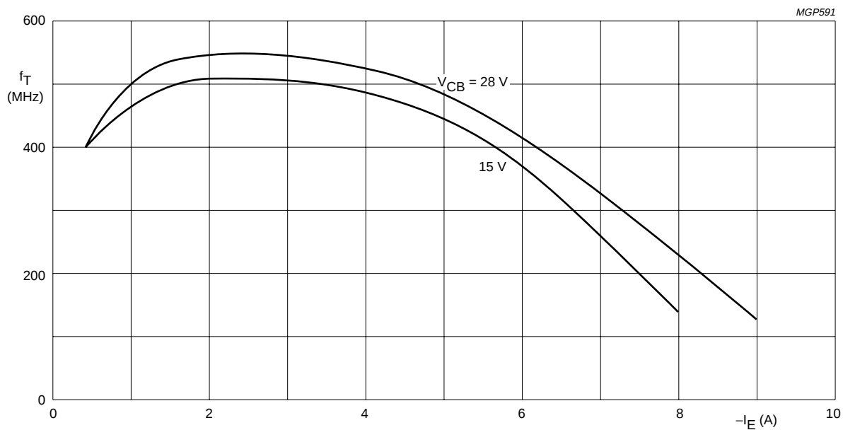
Fig.7 Typical values; f = 100 MHz; T_j = 25 °C.
