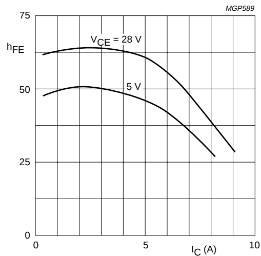
Fig.5 Typical values; T_j = 25 °C.
