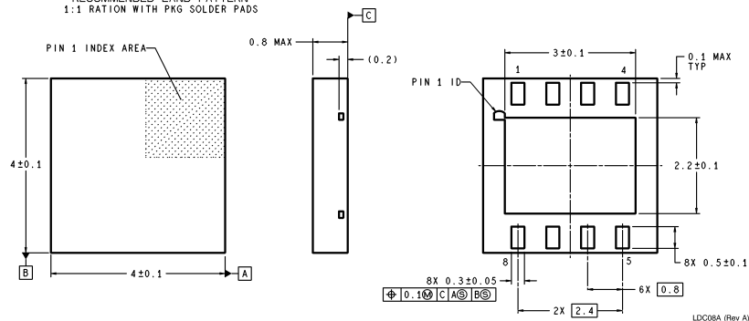
8-Lead LLP
