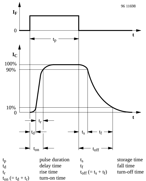
Figure 5. Switching times
