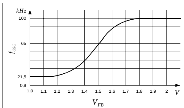
Figure 12 Frequency Dependence
