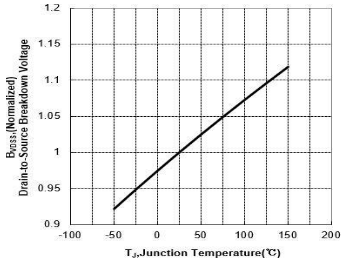
Figure 9 Typical Breakdown Voltage vs Junction Temperature
