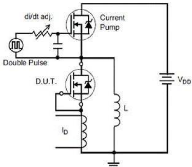
Figure 16 Diode Reverse Recovery Test Circuit
