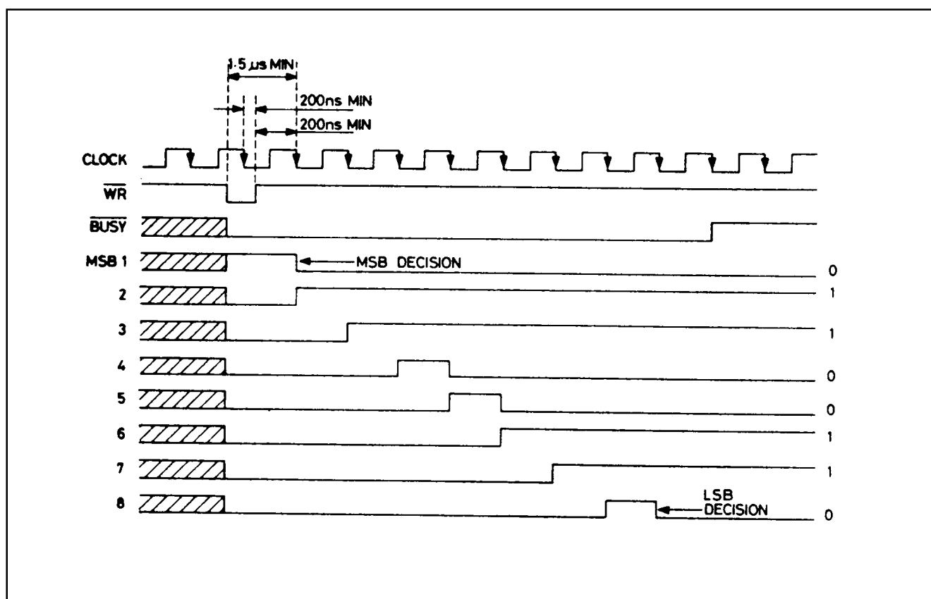
Fig.3 Timing diagram
