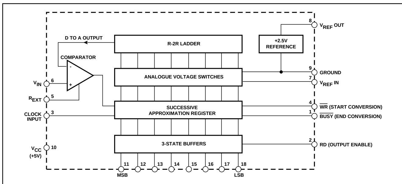
Fig.2 System diagram
