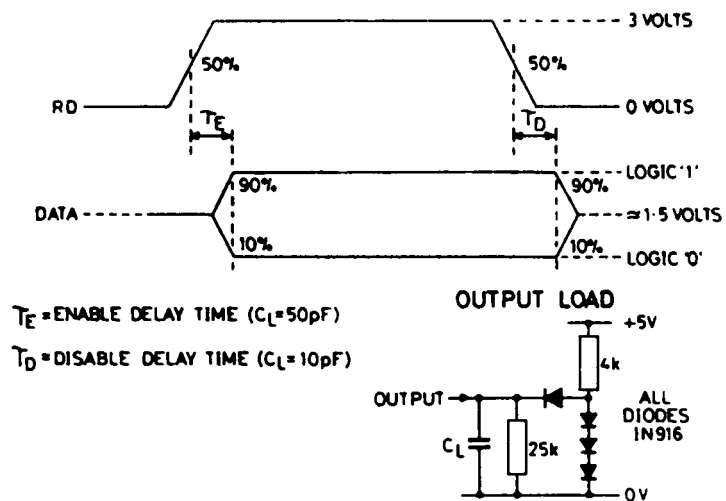
Fig.9 Output enable/disable waveforms
