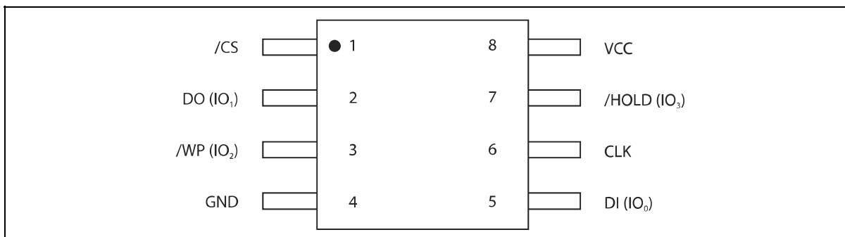
Figure 1a. W25Q16 Pin Assignments, 8-pin SOIC 208-mil (Package Code SS)
