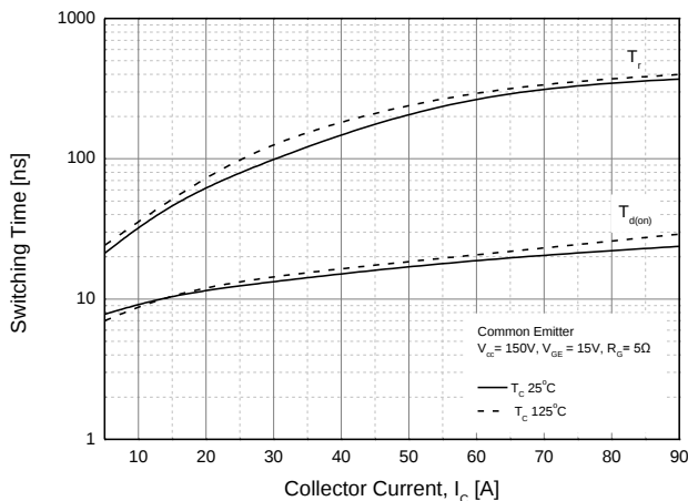
Fig. 8 Turn on time vs. collector current
