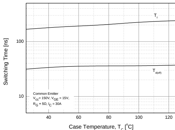
Fig. 12 Turn off time vs. Case temperature
