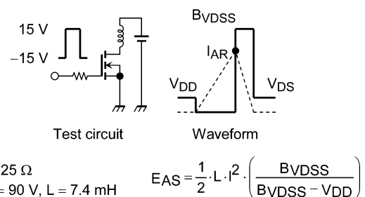
Fig. 8.16 Test Circuit/Waveform
