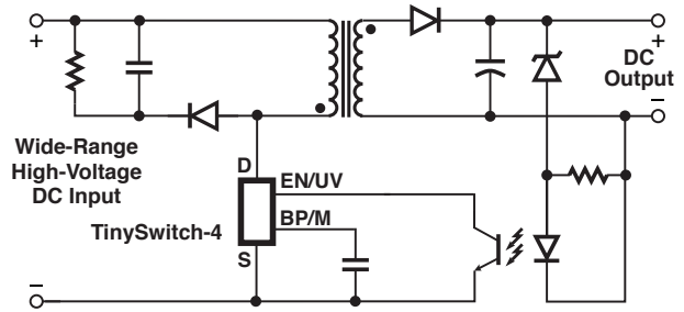
Figure 1. Typical Standby Application.
