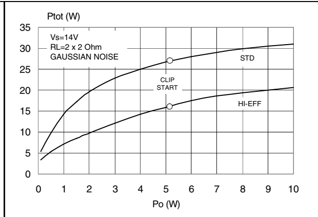
Figure 22. Power dissipation vs. average output power (Audio program simulation, 2Ω)
