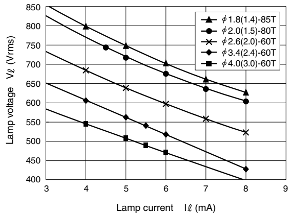
Lamp voltage - Lamp current (319 mm lamp)
