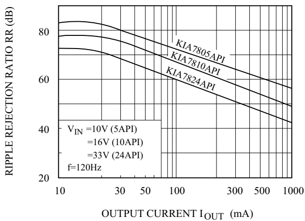
RR - I_{OUT}
