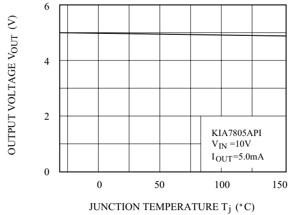
V_{OUT} - T_j
