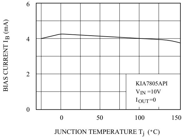
I_B - T_j
