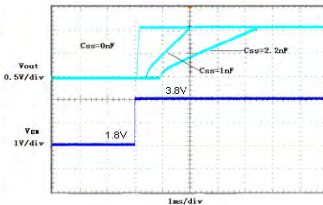
Figure 18 Turn-On Response
