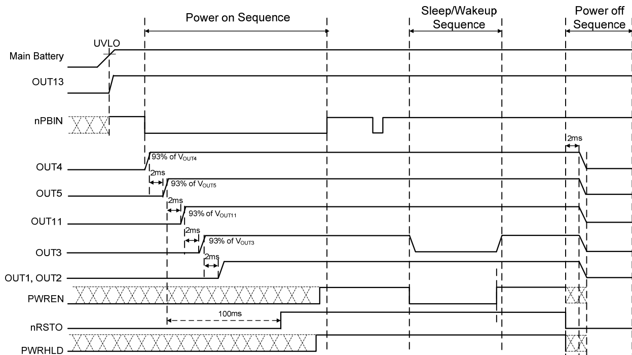
Figure 3: Power Control Sequence
