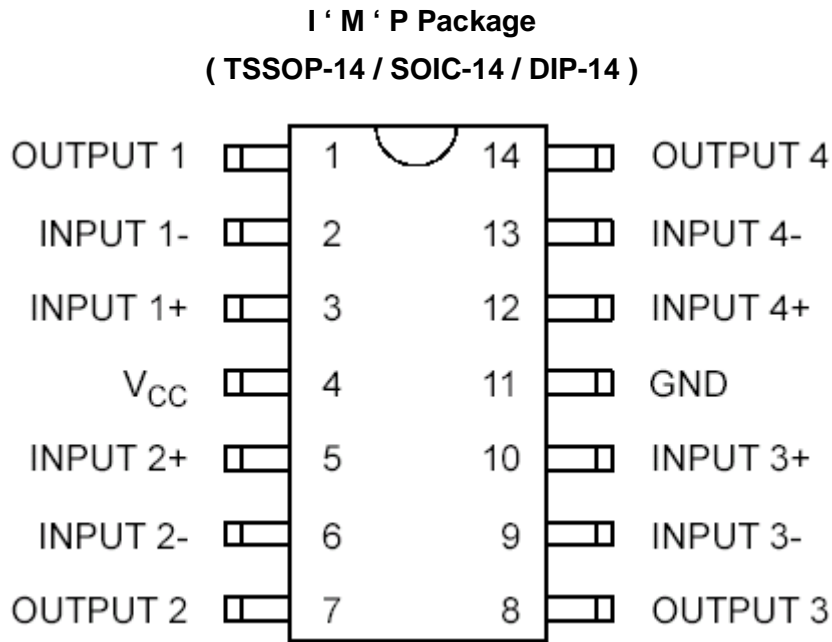
Figure 2. Pin Configuration of EC48324 (Top View)
