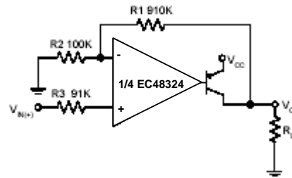
Figure 17. Power Amplifier
