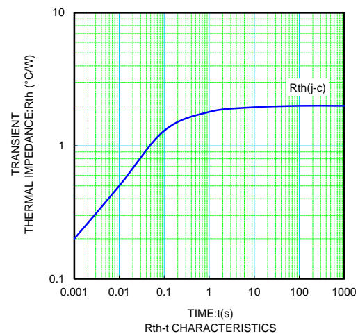
R_{th(j-c)} - t CHARACTERISTICS
