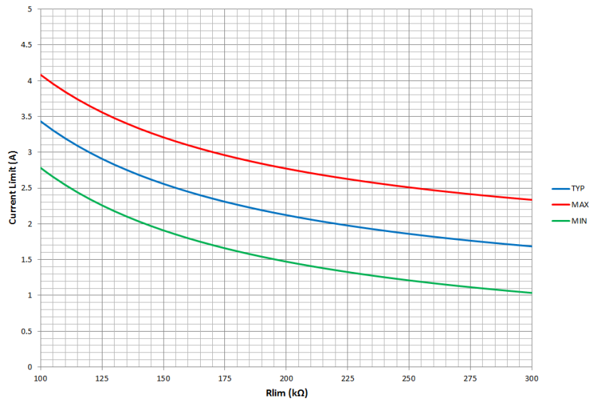
Figure 25. Buck 2
