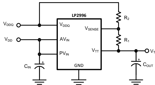
Figure 14. Decreasing VTT by Level Shifting
