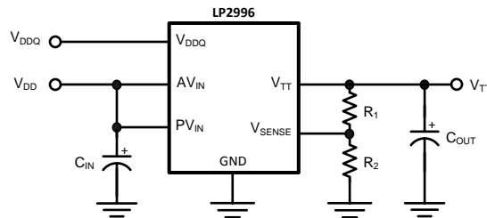
Figure 13. Increasing VTT by Level Shifting
