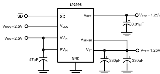
Figure 17. Typical SSTL-2 Application Circuit for Motherboards
