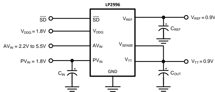
Figure 11. Recommended DDR-II Termination
