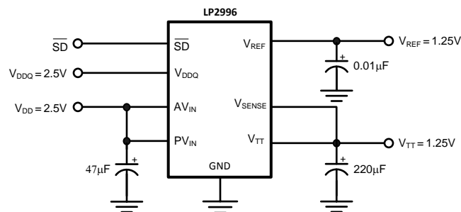
Figure 16. Typical SSTL-2 Application Circuit
