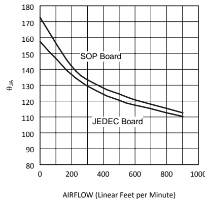
Figure 5. \theta_{\text{JA}} vs Airflow (SO-8)
