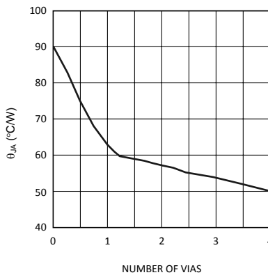
Figure 6. LLP-16 \theta_{JA} vs # of Vias (4 Layer JEDEC Board))
