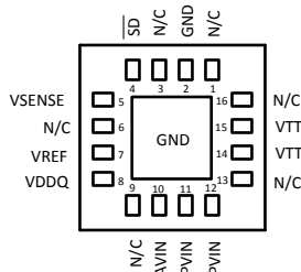
Figure 1. LLP-16 Layout (Top View)
