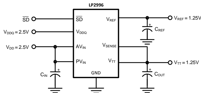
Figure 8. Recommended SSTL-2 Implementation
