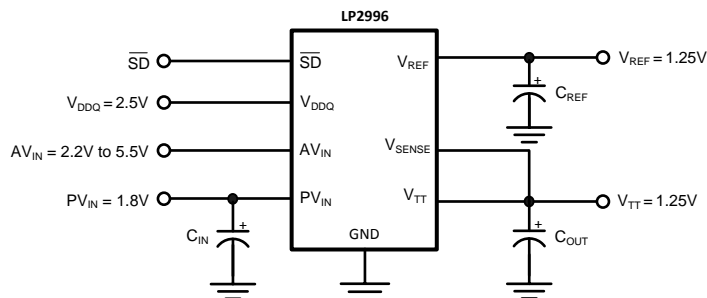
Figure 9. Lower Power Dissipation SSTL-2 Implementation
