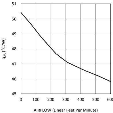
Figure 7. \theta_{JA} vs Airflow Speed (JEDEC Board with 4 Vias)
