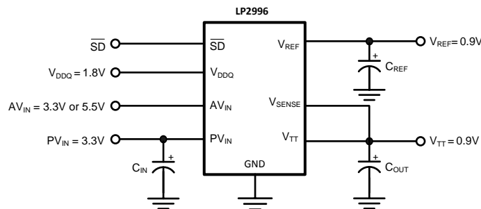
Figure 12. DDR-II Termination with higher voltage rails
