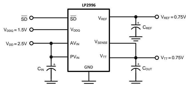
Figure 15. HSTL Application
