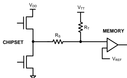
Figure 4. SSTL-Termination Scheme
