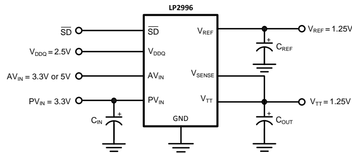
Figure 10. SSTL-2 Implementation with higher voltage rails
