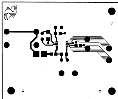
Figure 36. Bottom Layer
