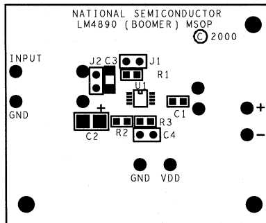
Figure 35. Top Layer
