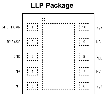
Figure 5. Top View Order Number LM4890LD See NS Package Number LDA10B
