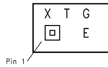
Figure 2. Top View X - Date Code T - Die Traceability G - Boomer Family E - LM4890IBP
