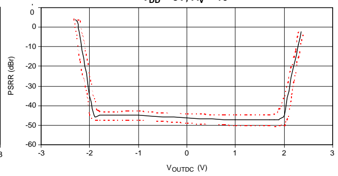
PSRR Distribution V_{DD} = 3V 217Hz, 200mvp-p, -30, +25, and +80°C
