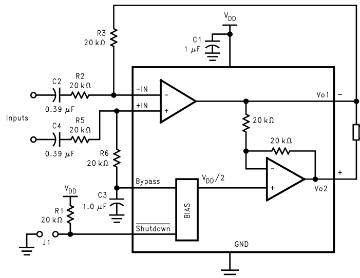
Figure 23. DIFFERENTIAL AMPLIFIER CONFIGURATION FOR LM4890
