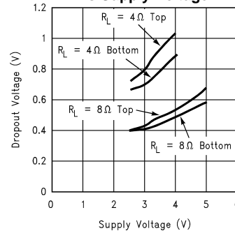
Clipping (Dropout) Voltage vs Supply Voltage
