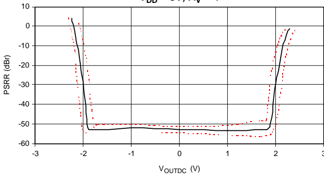
PSRR Distribution V_{DD} = 5V 217Hz, 200mvp-p, -30, +25, and +80°C
