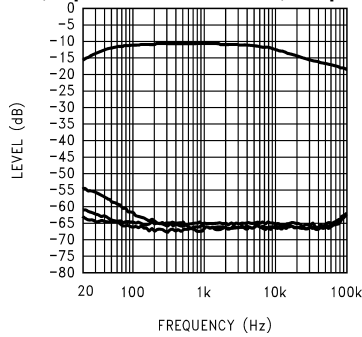
Figure 14. Top Trace = No Cap, Next Trace Down = 1\mu f Next Trace Down = 2\mu f , Bottom Trace = 4.7\mu f
