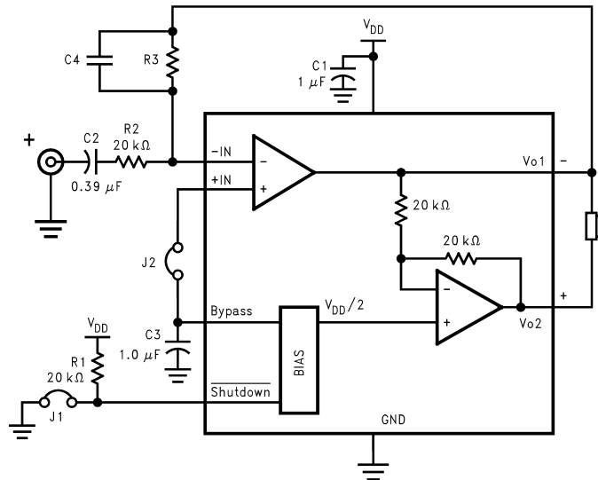
Figure 22. HIGHER GAIN AUDIO AMPLIFIER
