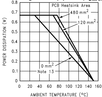
Power Derating - 9 bump \mu SMD ( P_{DMAX} = 670mW )
