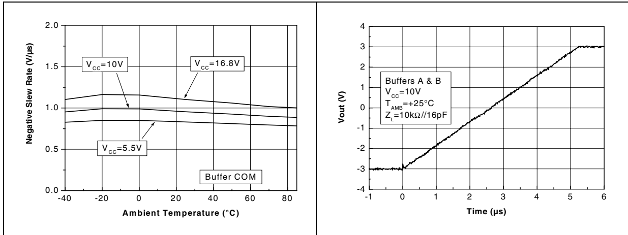
Figure 28. Large signal response - buffers A & B
