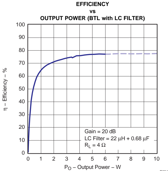
NOTE: Dashed line represents thermally limited region. Figure 22.
