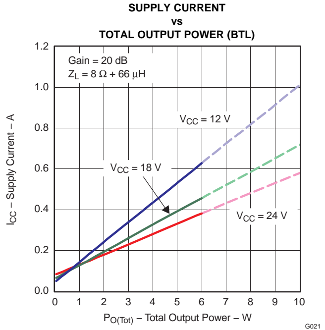
NOTE: Dashed lines represent thermally limited region. Figure 23.
