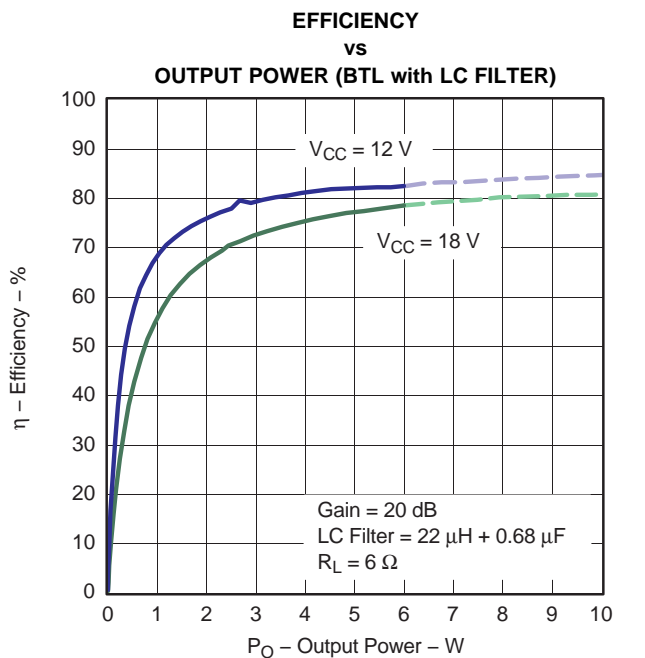
NOTE: Dashed lines represent thermally limited region. Figure 20.
