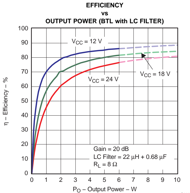
NOTE: Dashed lines represent thermally limited region. Figure 18.
