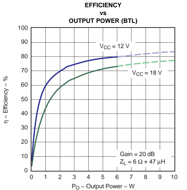
NOTE: Dashed lines represent thermally limited region. Figure 19.
