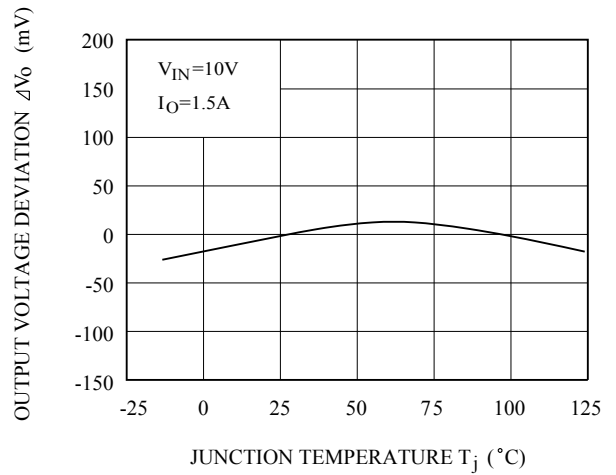
Fig.5-2 T_j - \Delta V_O (KIA378R08)
