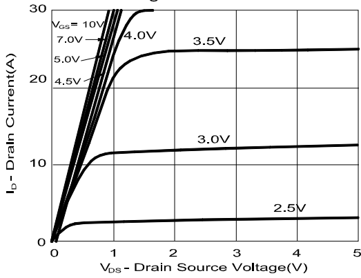
On-Region Characteristics
