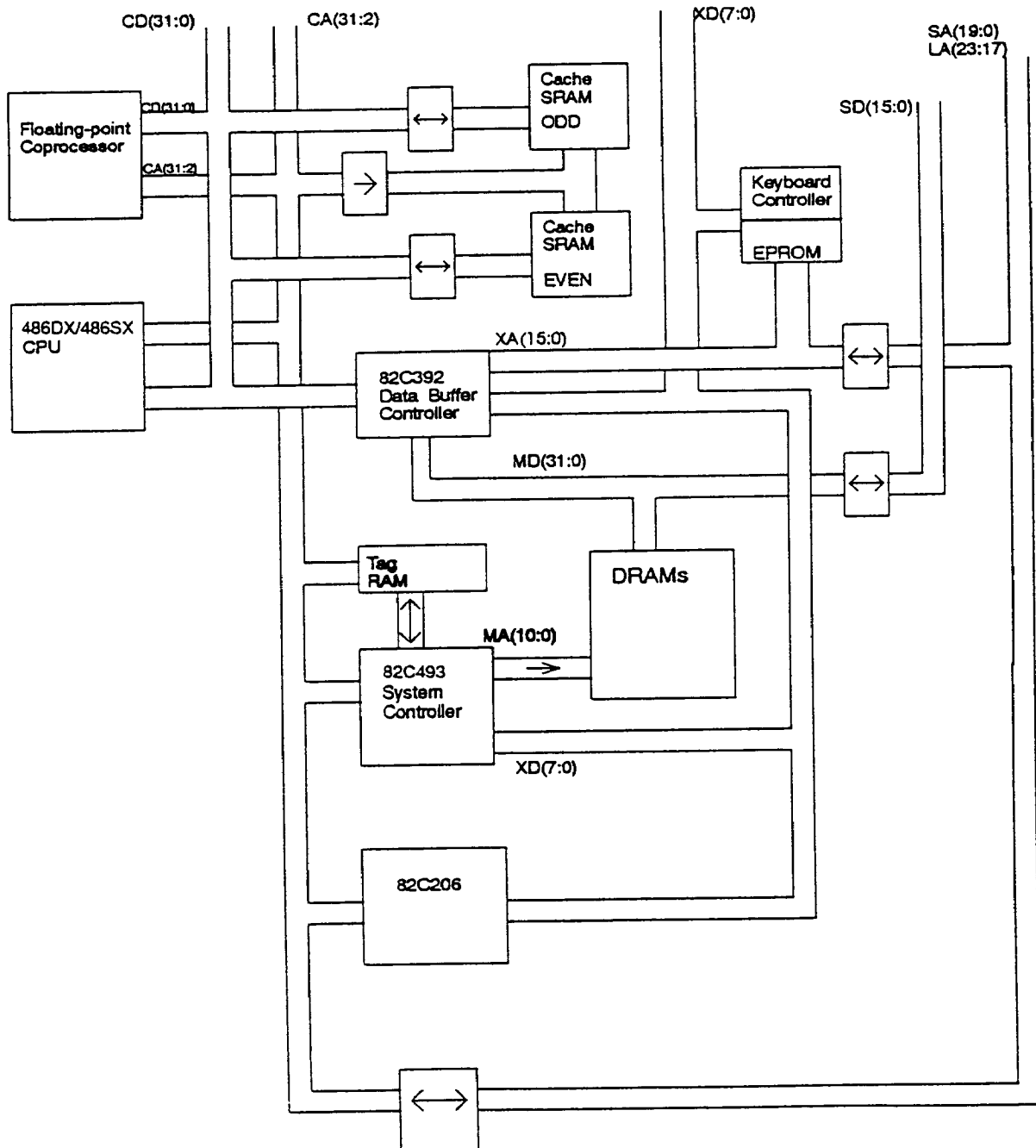
Figure 1. 486SXWB-Based System Block Diagram
