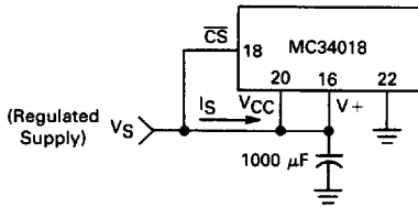
FIGURE 14 — ALTERNATE POWER SUPPLY CONFIGURATION
