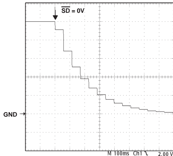
Figure 44. Differential Output With \overline{\text{FADE}} (Terminal 30) Held Low
