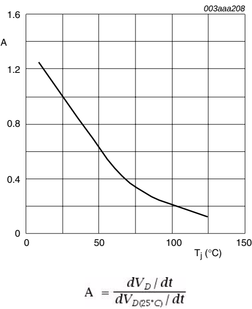
Fig 12. Normalized critical rate of rise of off-state voltage as a function of junction temperature; typical values
