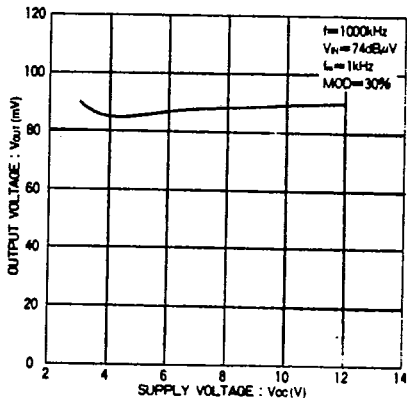
Fig. 26 AM detector output voltage vs. supply voltage
