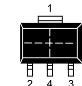
TOP VIEW SOT-223 PACKAGE See Mech. Drawings Section on Website
