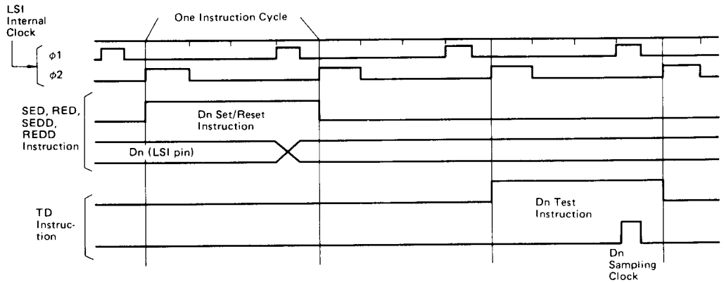
Figure 17 1-bit Discrete I/O Timing
