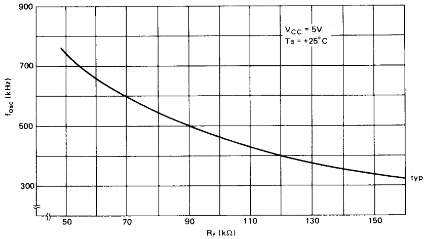
Figure 27 Typical Value of Oscillation Frequency vs. R f
