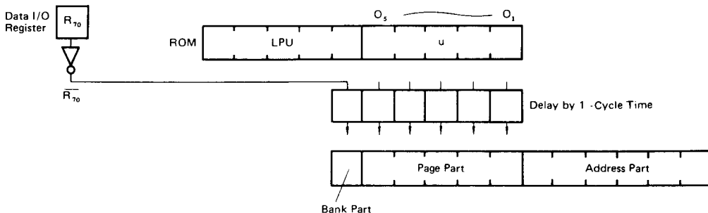
Figure 7 LPU Operation
