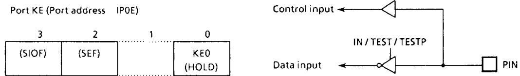
Figure 3-7. Port KE
