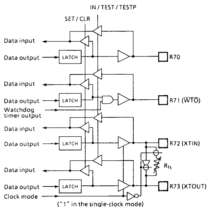
Figure 3-4. Port R7
