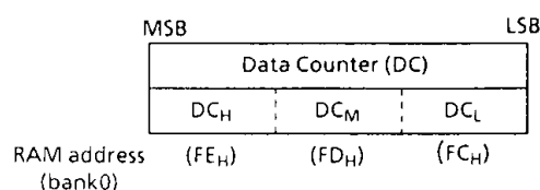
Figure 2-8. Data Counter
