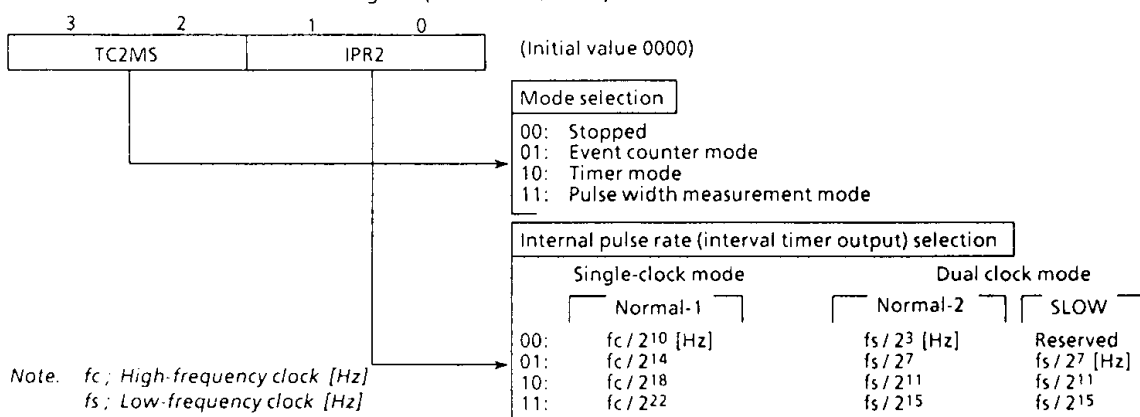
Figure 3-13. Timer/Counter Control Command Register
