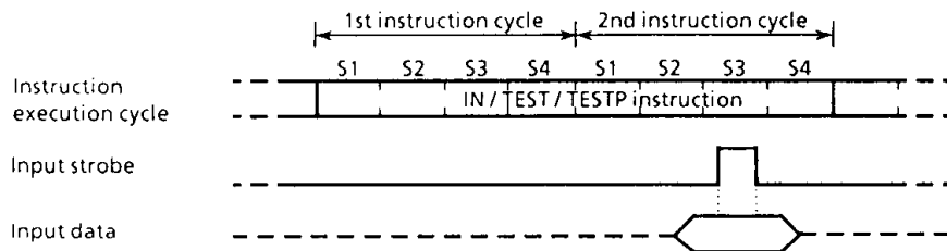
Figure 3-8. Input Timing
