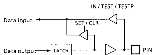
Figure 3-3. Ports R4, R5, R6
