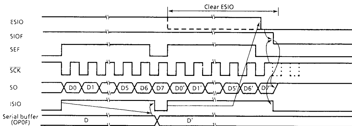
(b) External-clock-based operation
