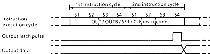
Figure 3-9. Output Timing
