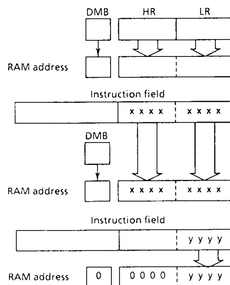
Figure 2-5. Addressing mode
