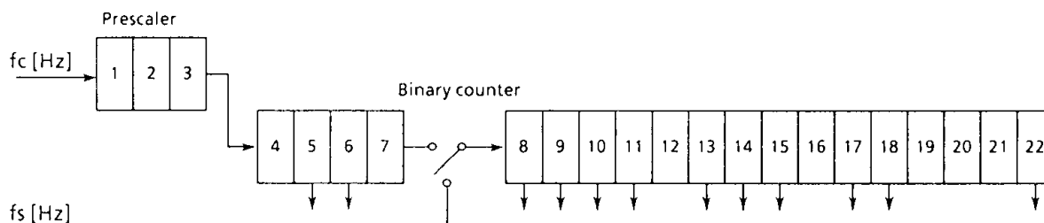
Figure 3-10. Configuration of Interval Timer
