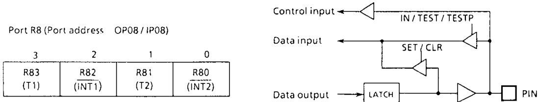
Figure 3-5. Port R8
