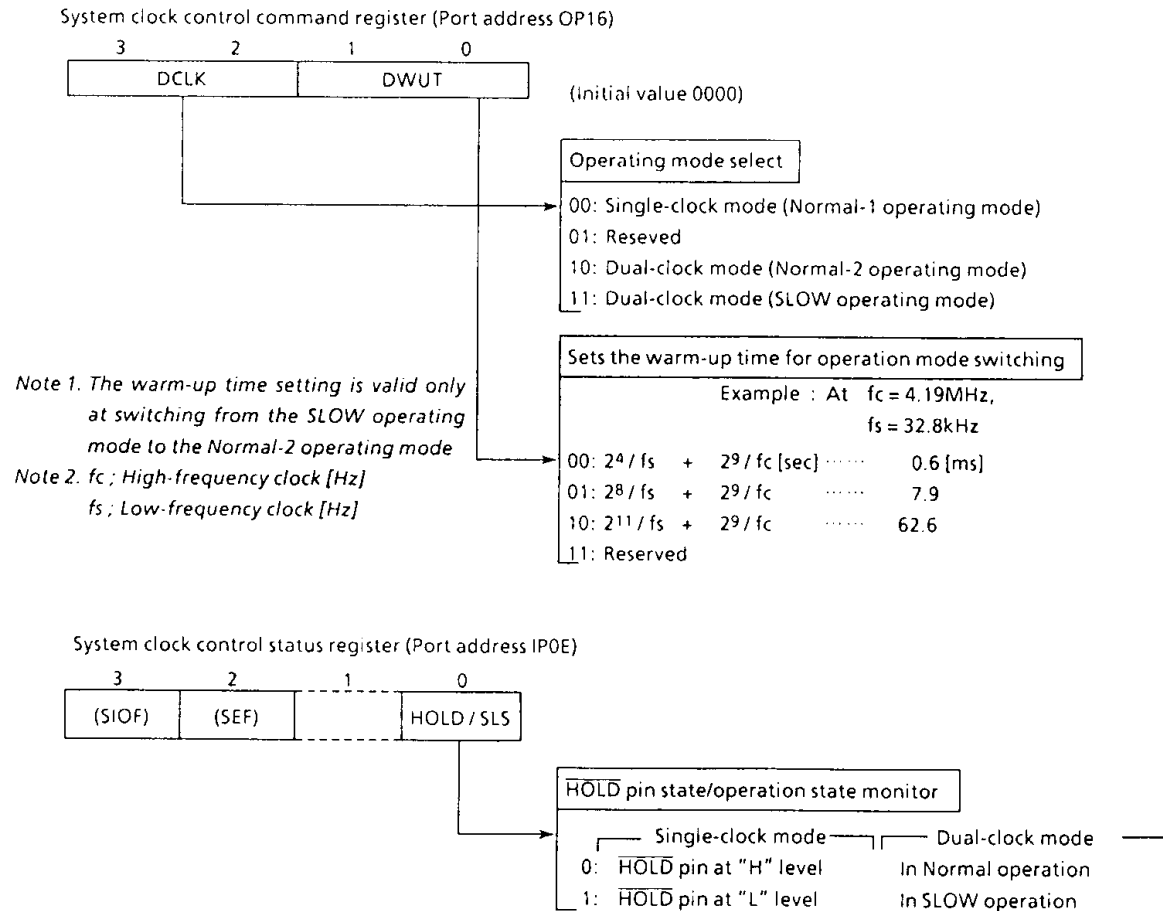
Figure 2-16. System Clock Control Command Register/Status Register
