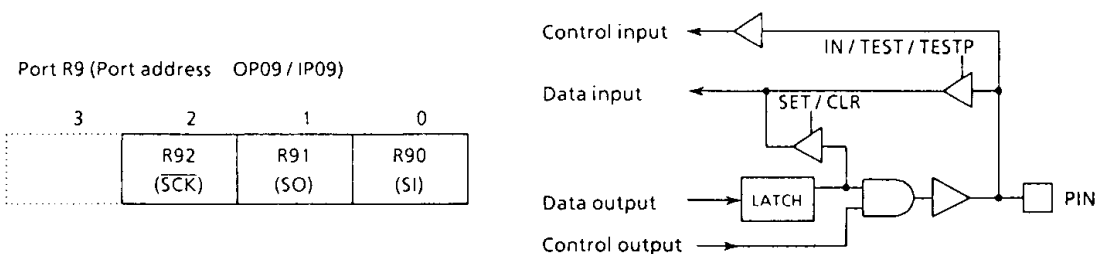
Figure 3-6. Port R9
