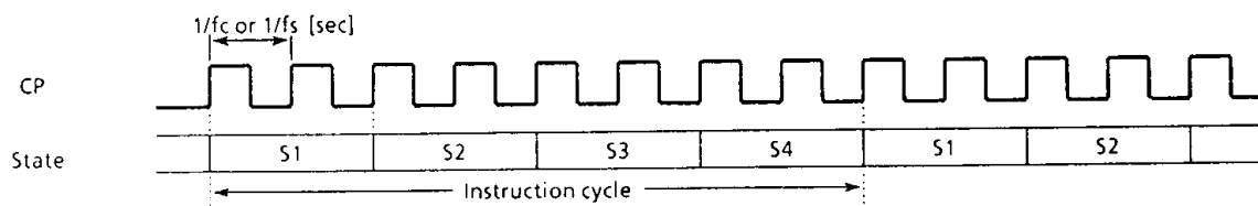
Figure 2-18. Instruction Cycle
