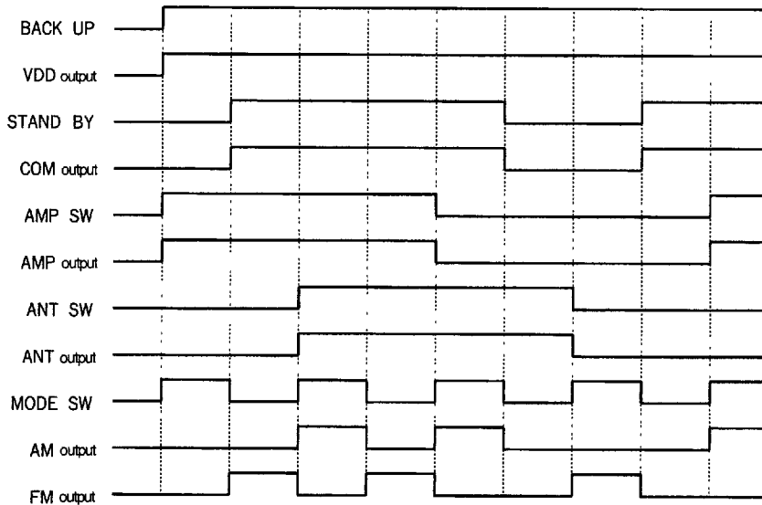
Figure 3 Timing chart
