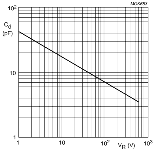
BYV27-500 and 600 f = 1 MHz; T j = 25 °C.
