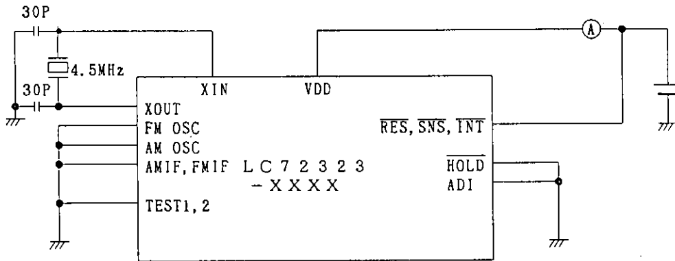
Figure 1 I_{DD} (2) in Hold Mode
