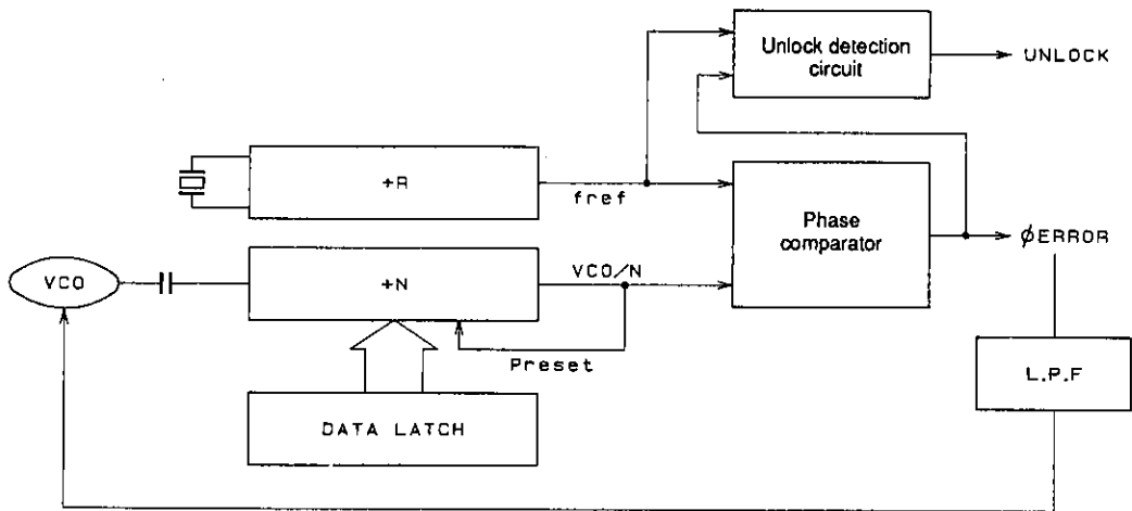
Figure 2 Circuit Structure
