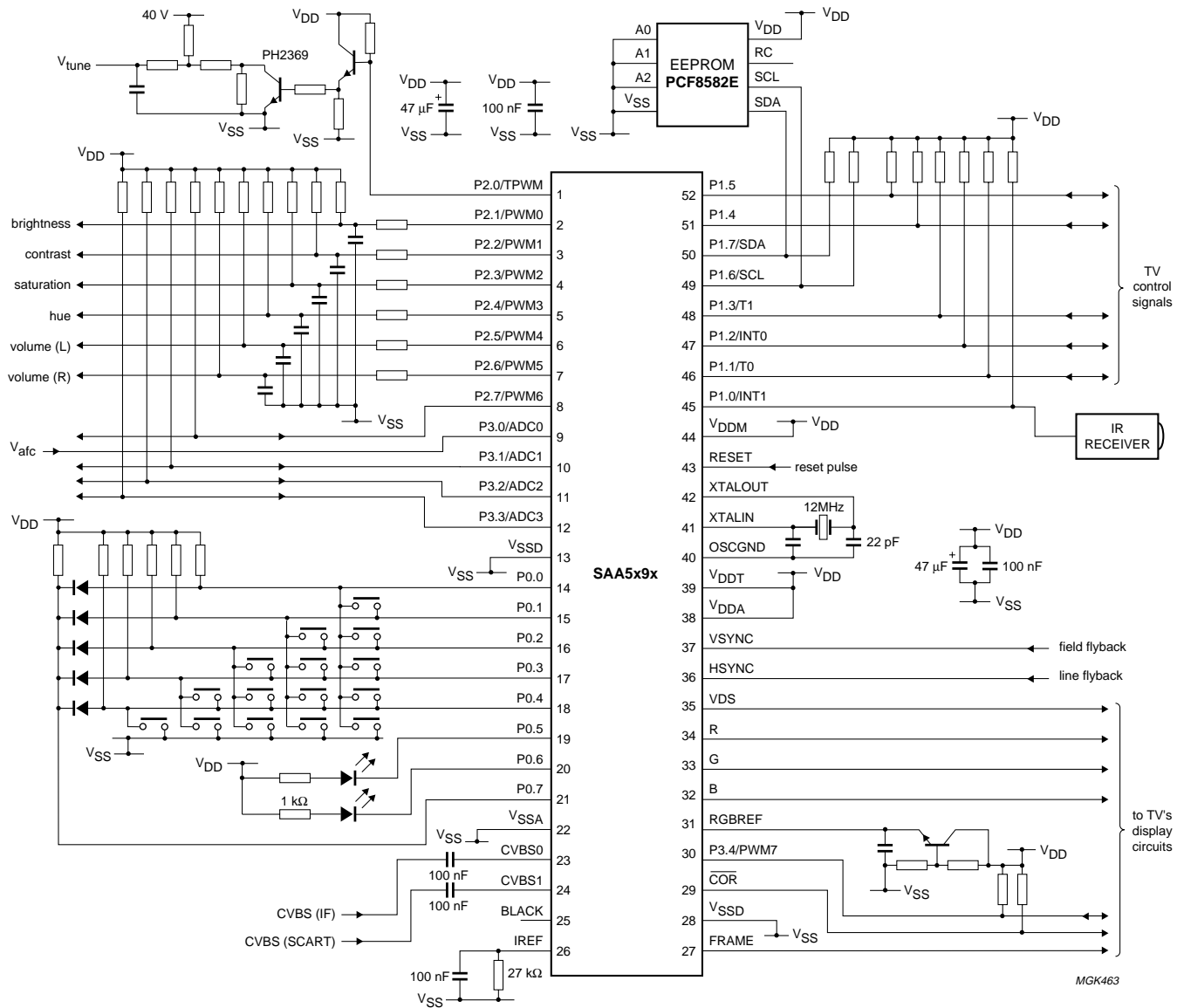
Fig.29 Application diagram.
