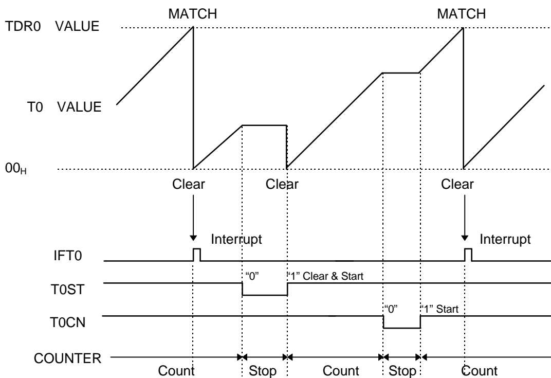
FIG 3.3.4 START/ STOP Control of Timer0
