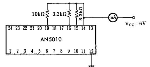
Test Circuit 16 ( I_{tot} )
