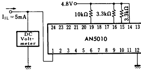
Test Circuit 1 ( V_{OL(K)} )
