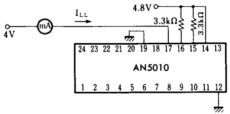
Test Circuit 14 ( I_{IH(OS)} )
