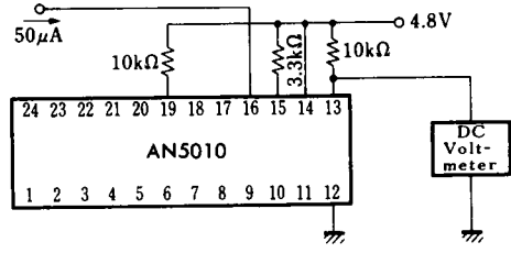
Test Circuit 8 ( I_{IH(CH)} )
