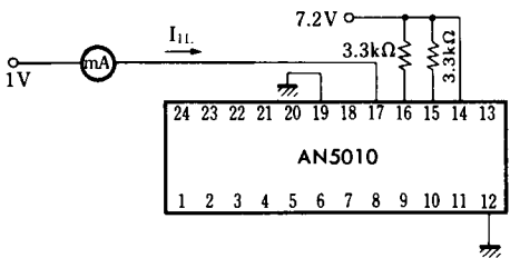
Test Circuit 13 ( I_{IL(OS)} )
