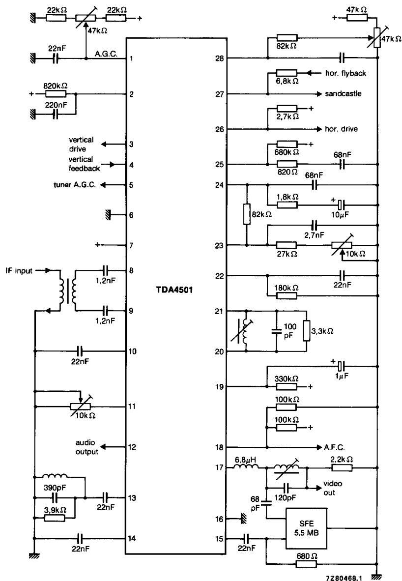
Fig. 2 Application diagram.
