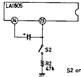
Fig.2 Forced Monaural Mode Setting Method
