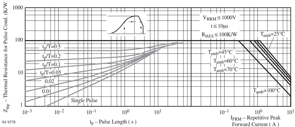
Figure 6. Thermal Response
