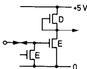
Fig. 7: Pin 10, Input/Output
